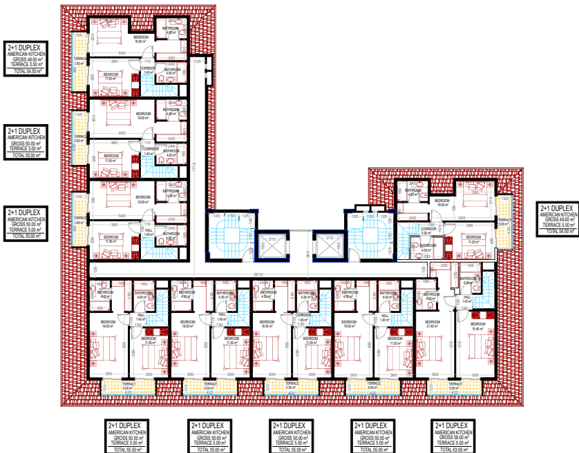
ROOF FLOOR PLAN
